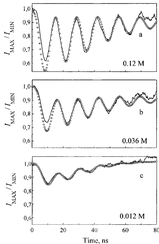
Figure 1. Quantum beats for the solutions of 10^{-3} M p -terphenyl- d_{14} in squalane and different concentrations of DPS-d_{10} : (a) 0.12 M; (b) 0.036 M; (c) 0.012 M. Solid lines indicate values taken from experiment, and circles represent those from simulation. The solution was held at ambient temperature.
